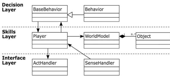
Fig. 2. (left) UML class diagram of the agent architecture used in the Senchans team. It shows the core classes of the system in the different layers. The modular design allows for easy extensibility. All sensory information from and to the robot is handled by the interaction layer. The information stored in structures of the skills layer, which also provides methods for predicting the future world state. These are used by classes in the decision layer to determine the best action of the agent for the current situation. (right) The HOAP-2 robot used in the Senchans team.
